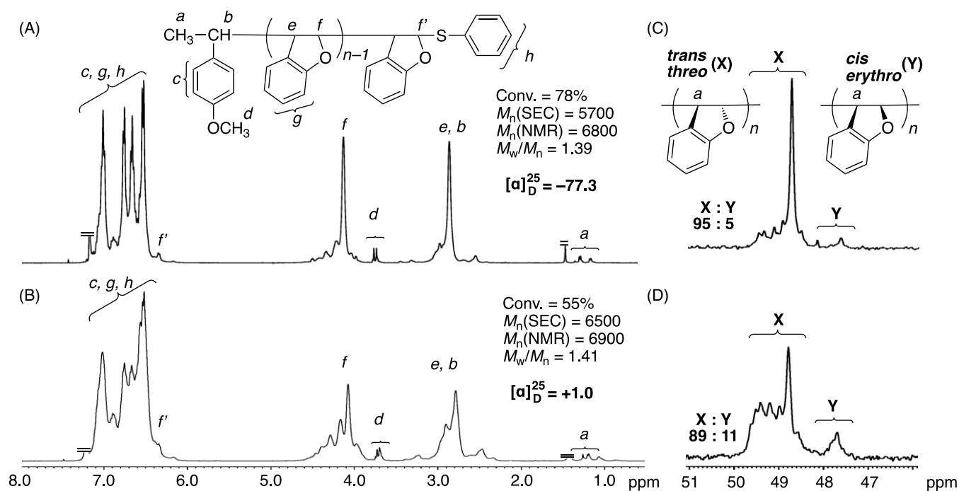
Figure 6. ^1\text{H} NMR (A, B) and ^{13}\text{C} NMR (C, D) spectra ( \text{CDCl}_3 , 55\text{ }^\circ\text{C} ) of the polymers obtained in asymmetric living cationic polymerization of BzF in toluene (A, C) and \text{CH}_2\text{Cl}_2 (B, D): [\text{BzF}]_0/[\text{CTAI}]_0/[\text{AlCl}_3]_0/[(R)\text{-}2\text{a}]_0 = 200/4.0/40/20 mM in toluene or \text{CH}_2\text{Cl}_2 at -78\text{ }^\circ\text{C} .
